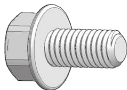
12 Flange Head Bolt M8-1.25 X 16
