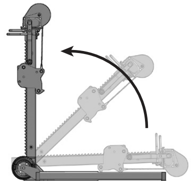
Tower Locking Pin (unlocked position)
